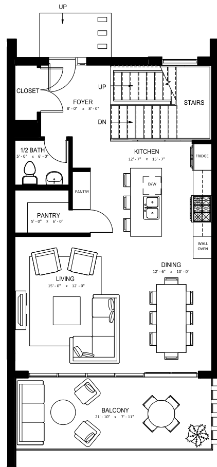
Main Floor - 753 Sq.Ft.
