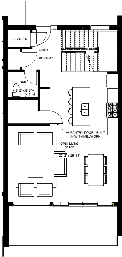
Main Floor - 753 Sq.Ft.
